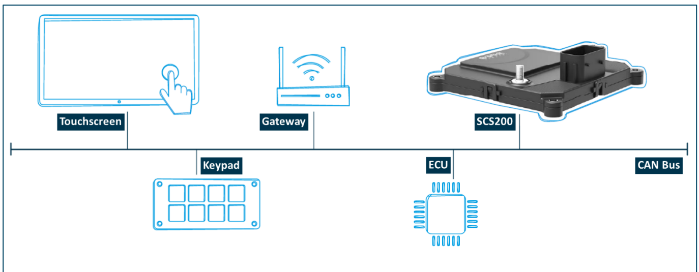
Figure 5: Example of a CAN network with an SCS200
