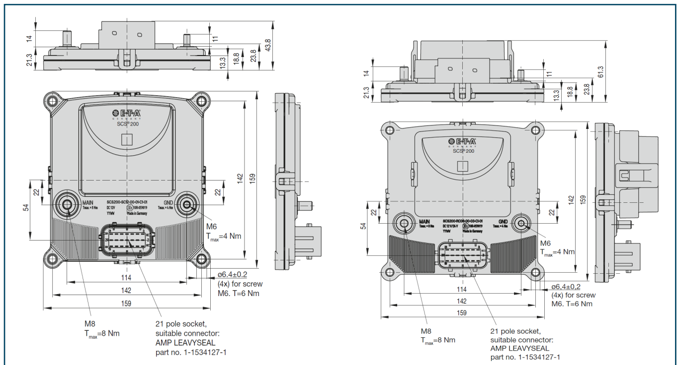
Figure 3: Dimensions SCS200-SC... (left) and SCS200-RC...(right)
