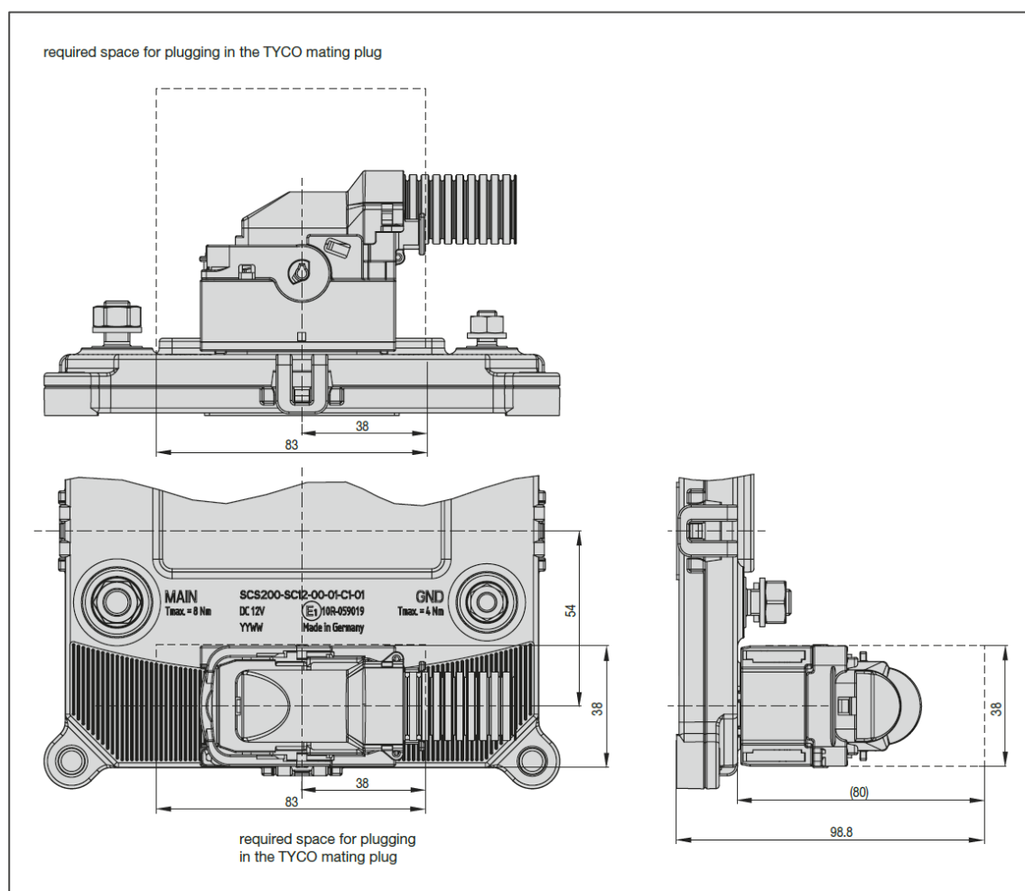
Figure 2: Required space for plugging in the Tyco mating plug
