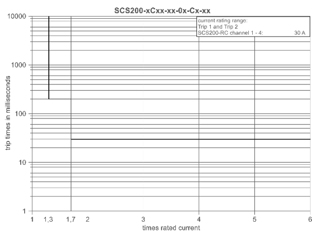
Figure 6: Overview of trip curves
