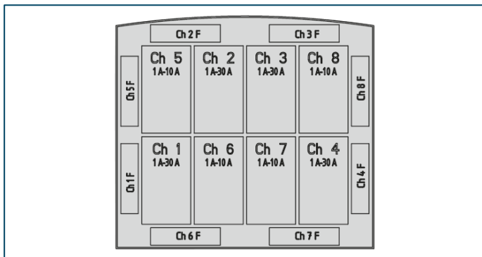
Figure 4: SCS200-RC... relay assignment
